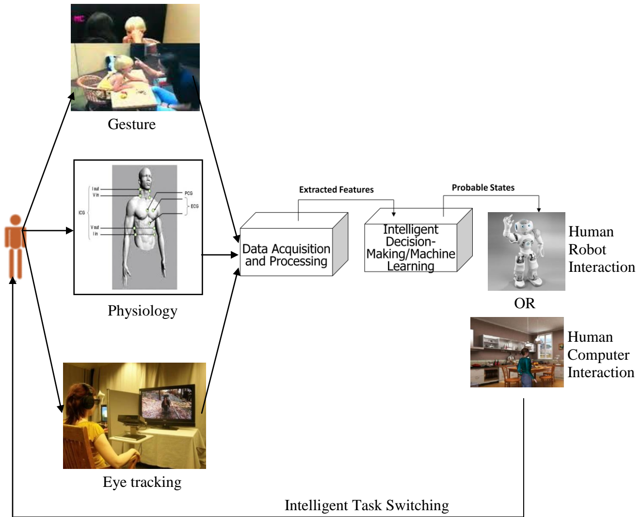
A typical Multi-modal Adaptive Architecture.
