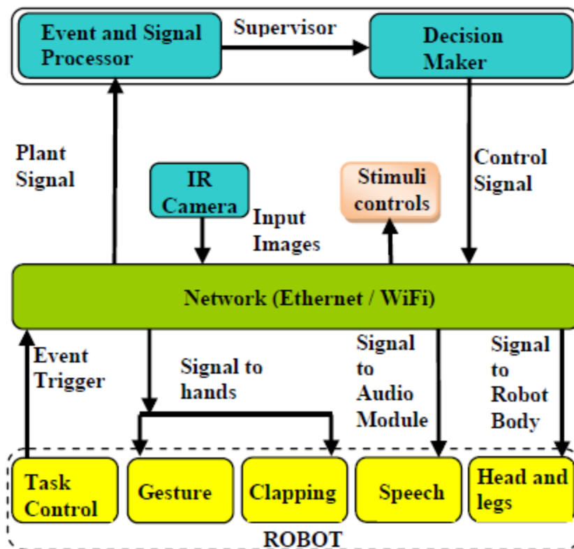
A typical System Architecture used.
